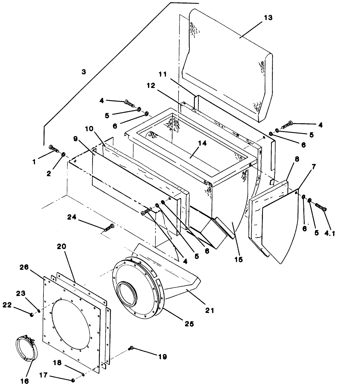
Figure 46. Exhaust Duct
